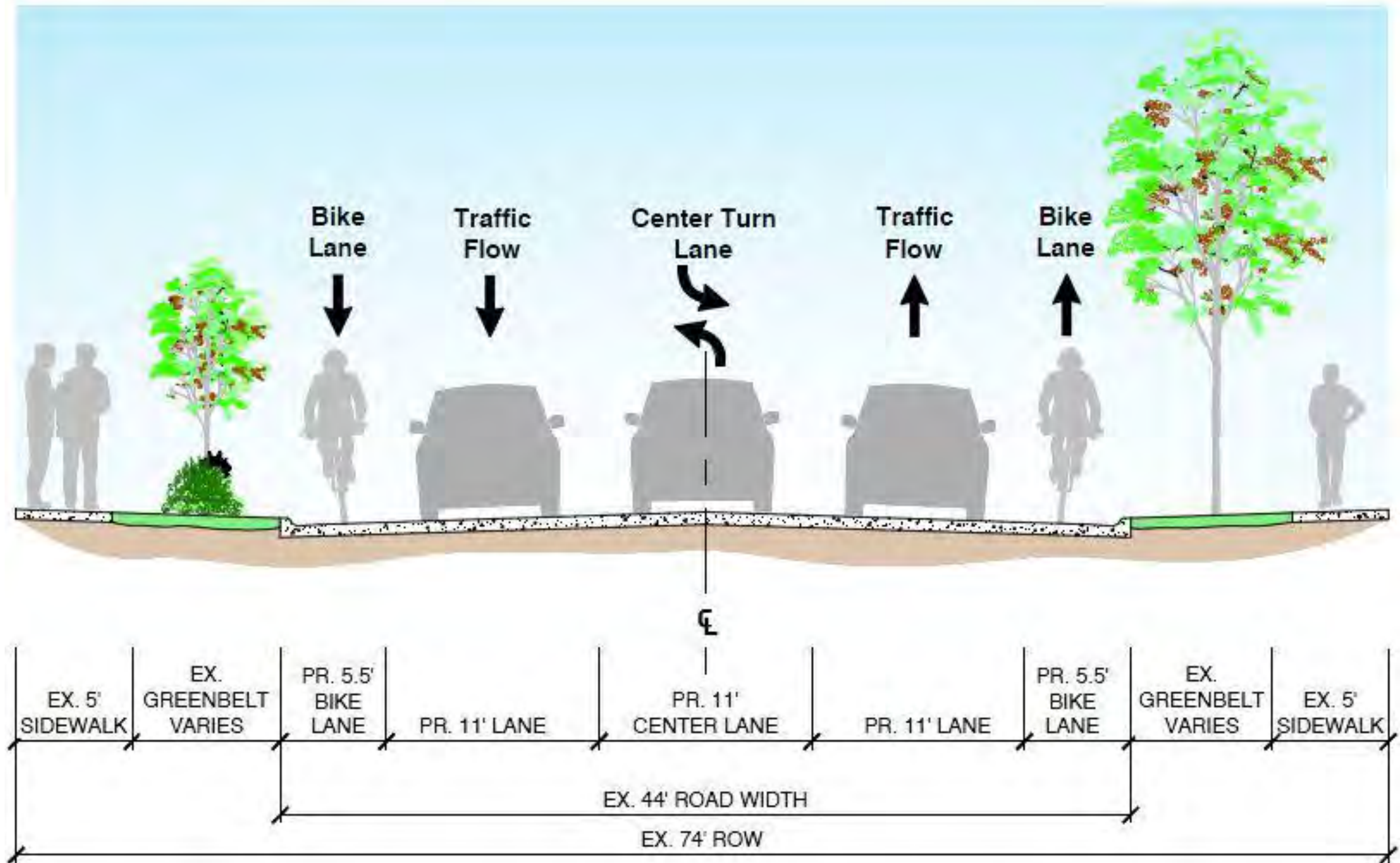
Proposed Cross Section Convert 4-lane section into 3-Lanes with Bike lanes
